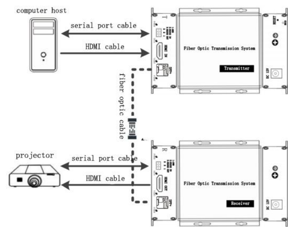
The connection diagram is for reference only
